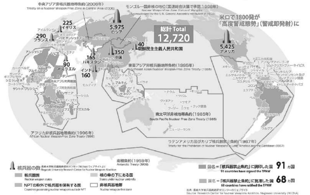
Number of Nuclear Weapons in the world, Nuclear-Weapon-Free Zones, and countries that have signed or ratified TPNW.
